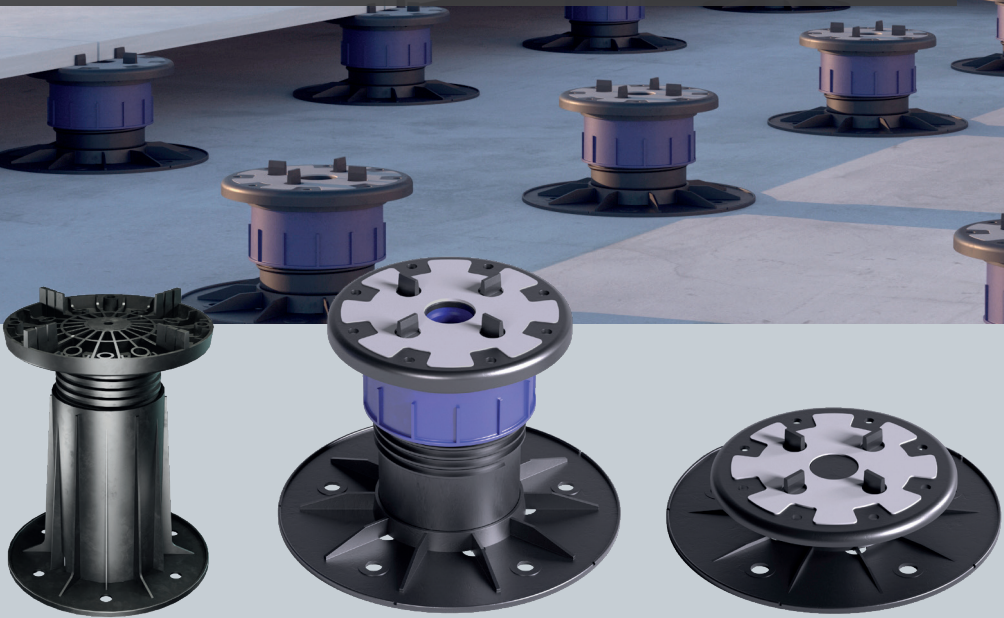
BSP
